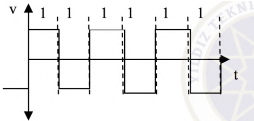
Figure 4.6 Polar NRZ-L and NRZ-I schemes
