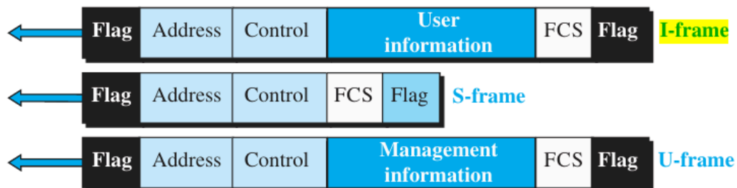
Figure 11.16 HDLC frames
