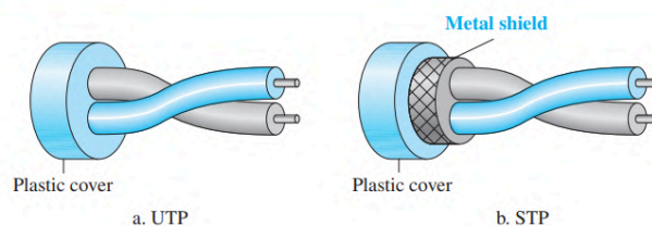
Figure 7.4 UTP and STP cables
