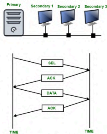
Figure : Select Mode
