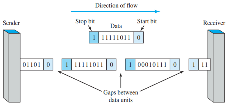
Figure 4.34 Asynchronous transmission
