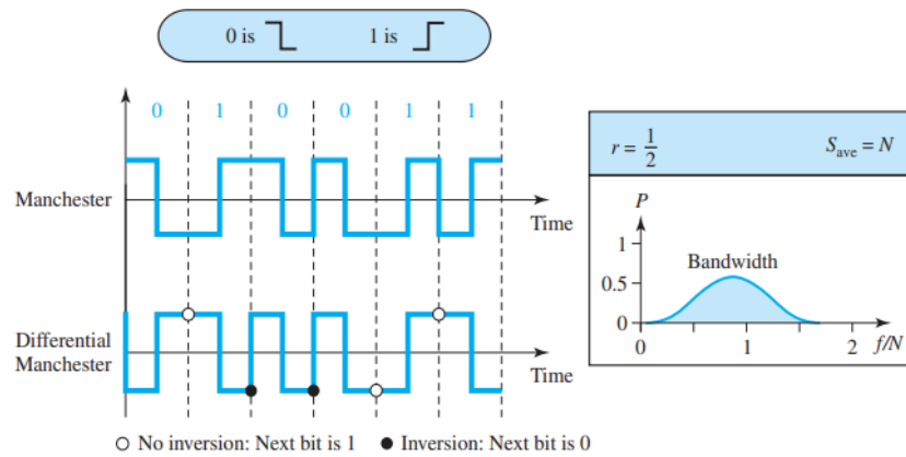
Figure 4.8 Polar biphas: Manchester and differential Manchester schemes
