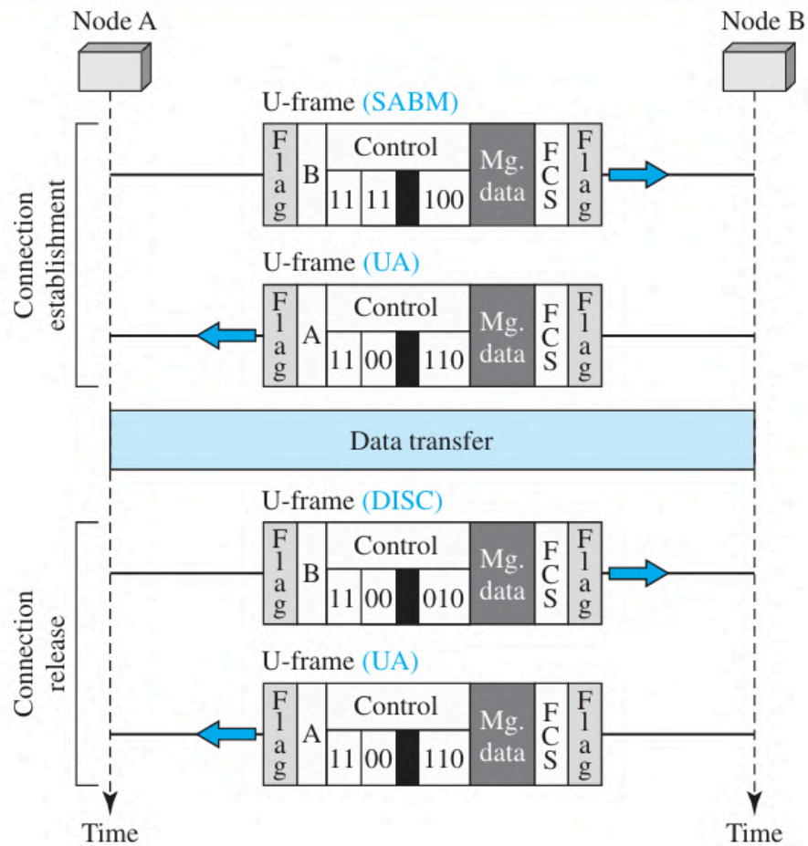
Figure 11.18 Example of connection and disconnection
