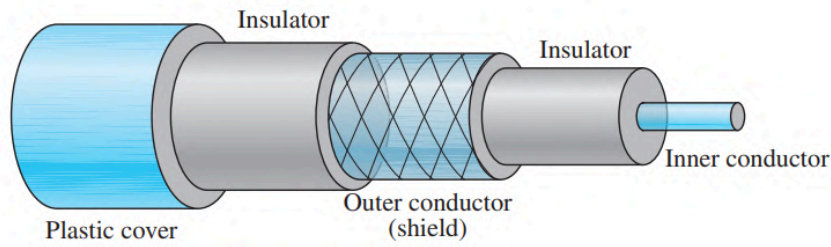
Figure 7.7 Coaxial cable
